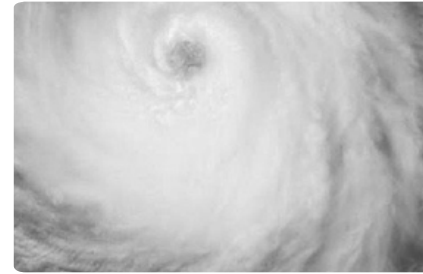
Credit NOAA/RAMMB
